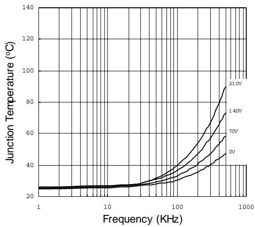
Figure 44. R21094S vs Frequency (IRFBC40) R gate = 15Ω, V CC = 15V
