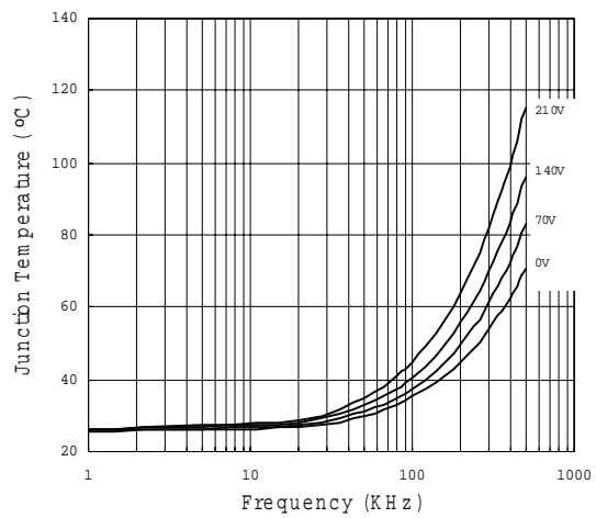
Figure 45. R21094S vs Frequency (IRFPE50) R gate = 10Ω, V CC = 15V
