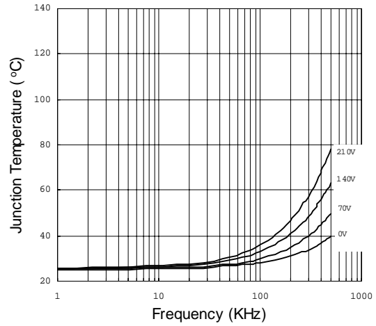
Figure 43. R21094S vs Frequency (IRFBC30) R gate = 22Ω, V CC = 15V
