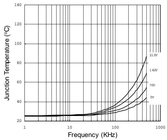
Figure 35. R2109S vs Frequency (IRFBC30) R gate = 22Ω, V CC = 15V
