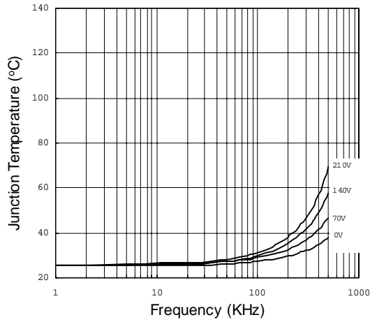
Figure 42. IR21094S vs Frequency (IRFBC20) R gate = 33Ω, V CC = 15V
